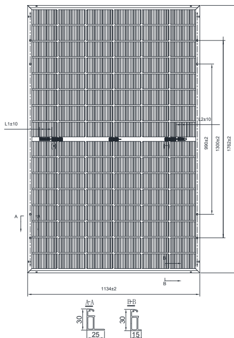
Aluminum Frame
