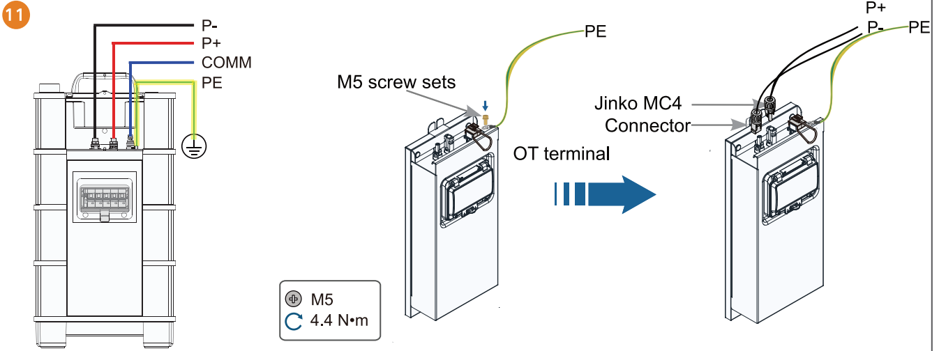
Connection Diagram
